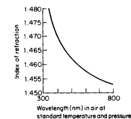
Index of refraction variation for fused quartz
