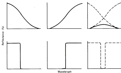
Subtractive colour mixing (Wasserman 2.2)
