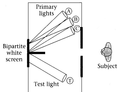
The color matching experiment (Wandell, 4.10)
