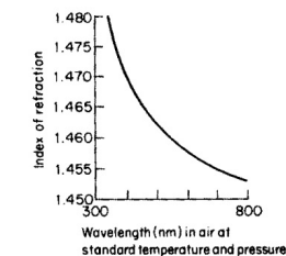
Index of refraction variation for fused quartz
