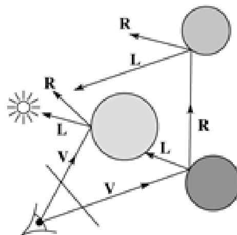
Reflection rays
