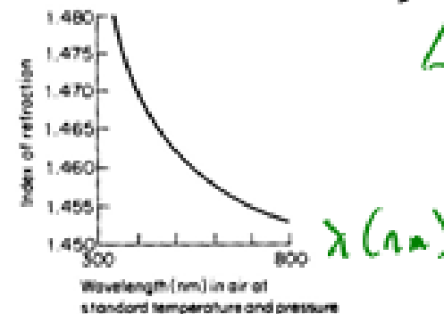
Index of refraction variation for fused quartz
