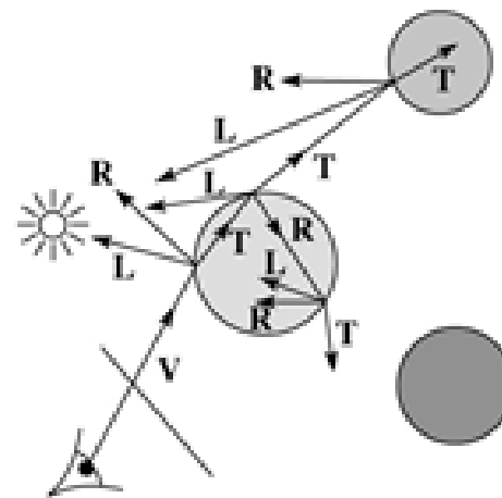
Refracted rays
