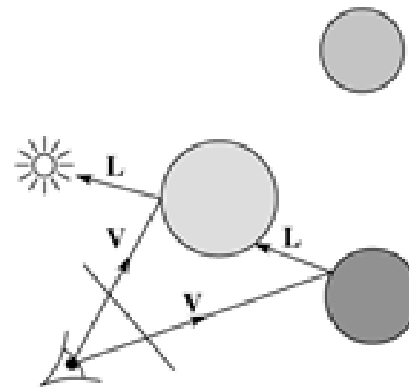
Shadow rays
