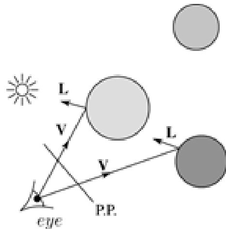
Primary rays
