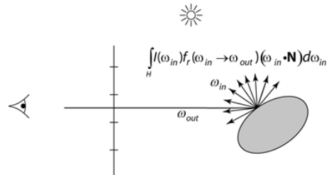
Reflection anti-aliasing
