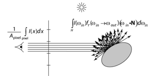
Pixel and reflection anti-aliasing
