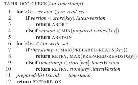
Figure 8: Validation function for checking for OCC conflicts on Prepare . PREPARED-READS and PREPARED-WRITES get the proposed timestamps for all transactions that the replica has prepared and read or write to key , respectively.
