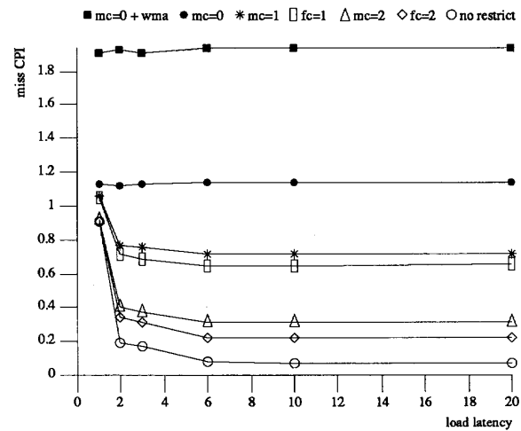
Figure 4-8: Baseline Miss CPI for tomcatv
