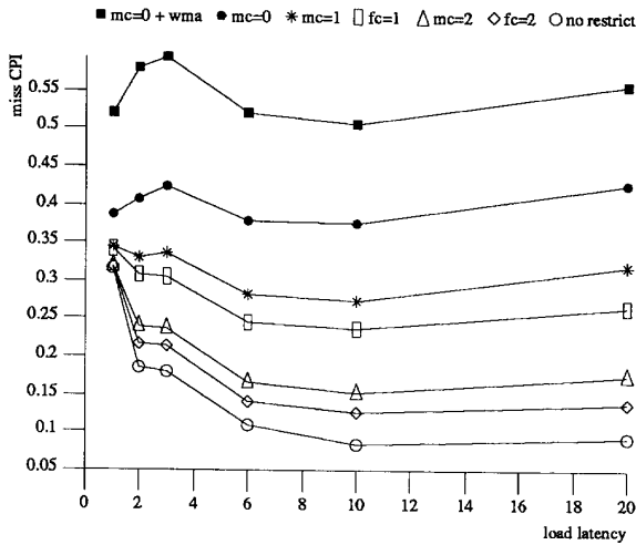
Figure 5-2: Miss CPI for doduc with 16 byte lines
