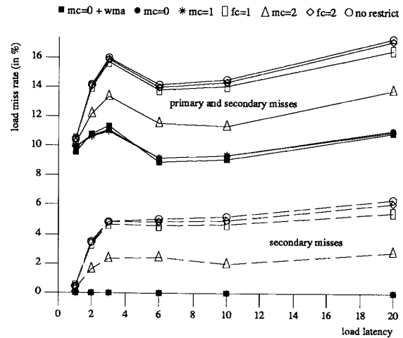
Figure 4-4: Baseline Miss rate for doduc
