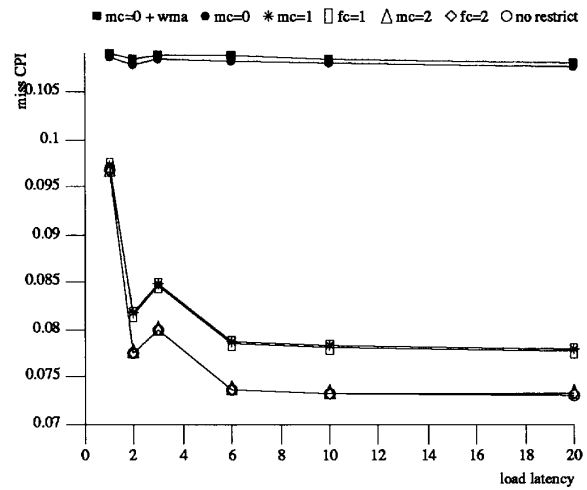
Figure 4-7: Baseline Miss CPI for eqntott
