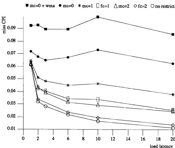
Figure 5-1: Miss CPI for doduc with a 64KB data cache
