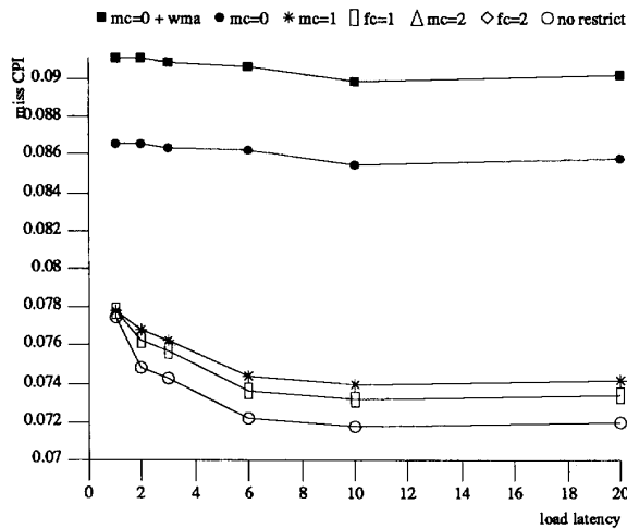
Figure 4-6: Miss CPI for xdisp with a fully associative cache
