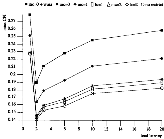
Figure 4-5: Baseline Miss CPI for xdisp
