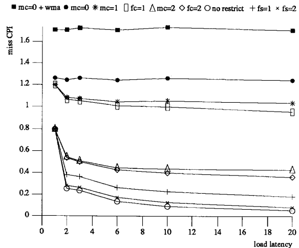
Figure 4-11: Baseline Miss CPI for su2cor
