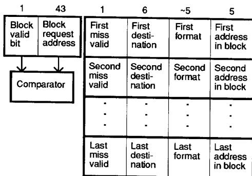
Figure 2-2: Explicitly addressed MSHR fields
