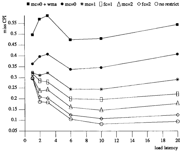
Figure 4-1: Baseline Miss CPI for doduc
