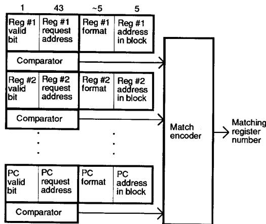
Figure 2-3: Inverted MSHR organization
