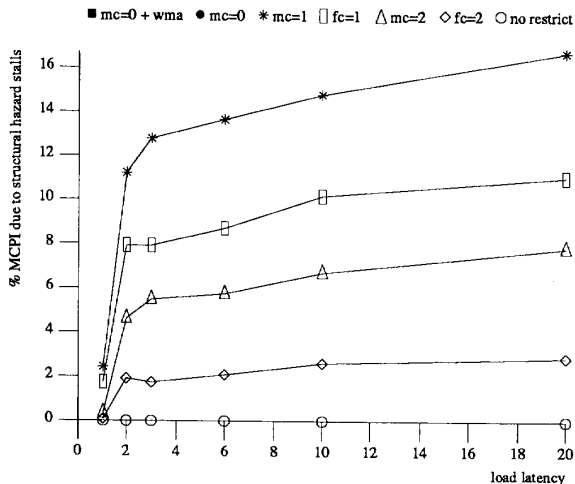
Figure 4-3: Stall cycle breakdown for doduc
