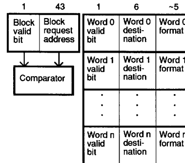
Figure 2-1: Basic implicitly addressed MSHR fields
