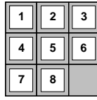
Goal State
