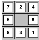
Start State
