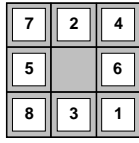
Start State
