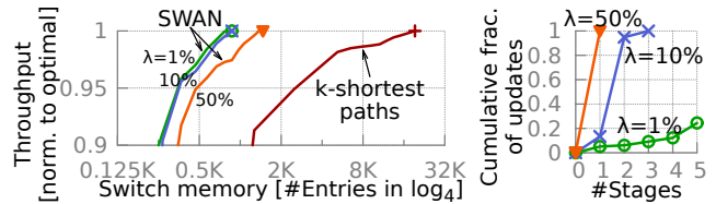
Figure 16: SWAN needs fewer rules to fully exploit network capacity (left). The number of stages needed for rule changes is small (right).
