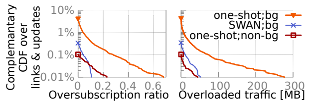
Figure 15: Link oversubscription during updates.
