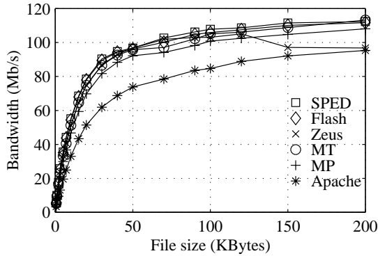
Figure 6: Solaris single file test — On this trivial test, server architecture seems to have little impact on performance. The aggressive optimizations in Flash and Zeus cause them to outperform Apache.
