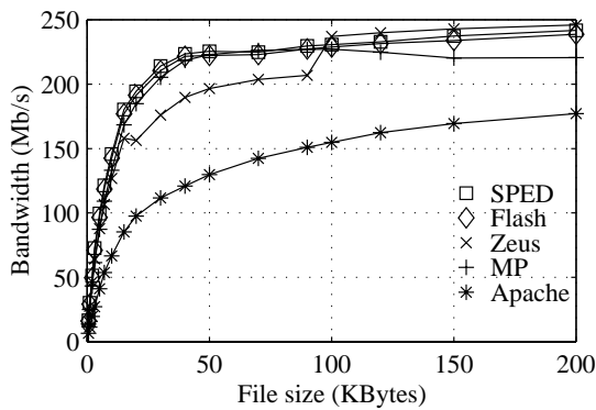
Figure 7: FreeBSD single file test — The higher network performance of FreeBSD magnifies the difference between Apache and the rest when compared to Solaris. The shape of the Zeus curve between 10 kBytes and 100 kBytes is likely due to the byte alignment problem mentioned in Section 5.5.
