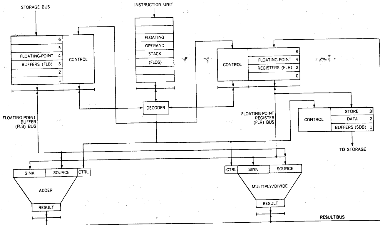
Figure 1 Data registers and transfer paths without CDB.
