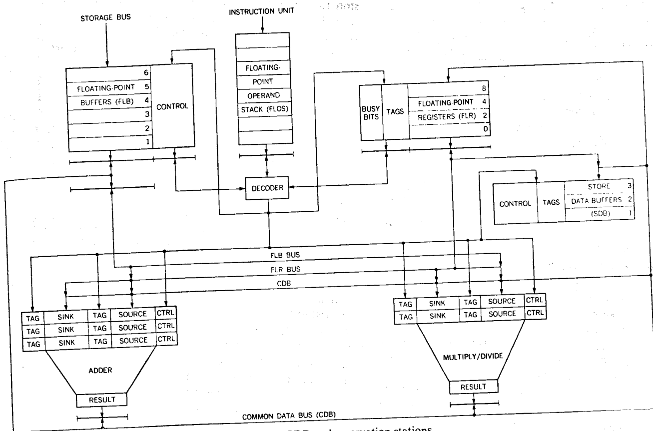
Figure 4 Data registers and transfer paths, including CDB and reservation stations.
