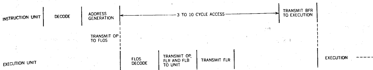
Figure 2 Timing relationship between instruction unit and FLOS decode for the processing of one instruction.
