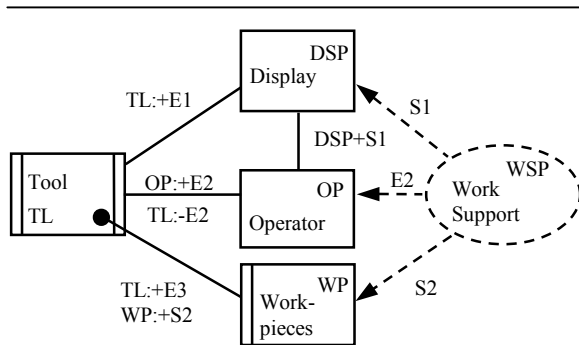
Figure 11 Composite Frame: Visible Workpieces
