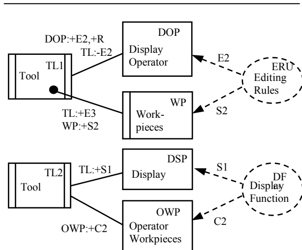
Figure 12 Decomposition of Visible Workpieces Frame
