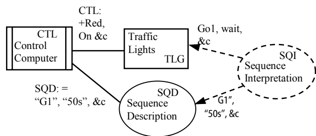
Figure 6 Flexible Traffic Lights Problem
