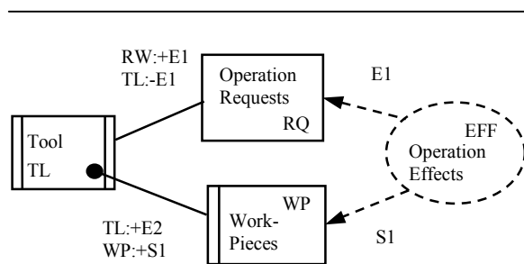
Figure 5 Elementary Frame: Simple Workpieces
