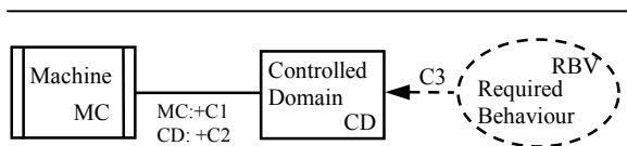
Figure 2 Elementary Frame: Simple Control
