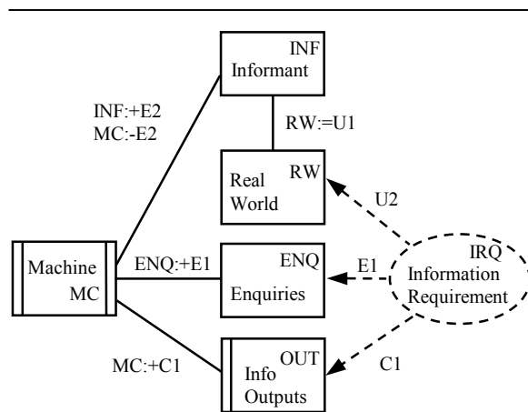
Figure 8 Composite Frame: Static IS with Informant
