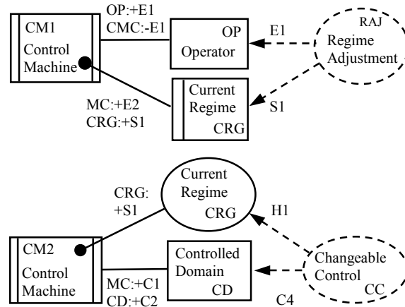
Figure 10 Decomposition of Simple Control Frame Under Operator's Regime
