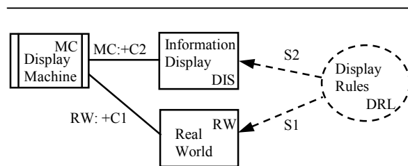
Figure 4 Elementary Frame: Information Display
