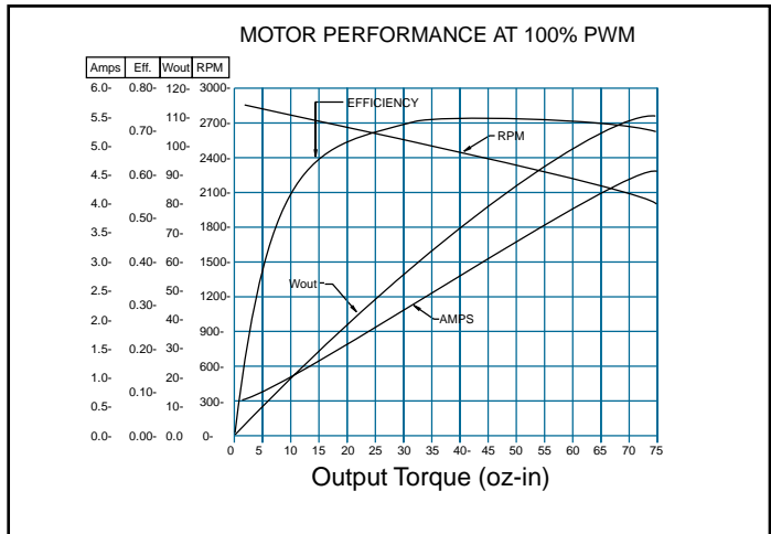
Motor Performance at 100% PWM
