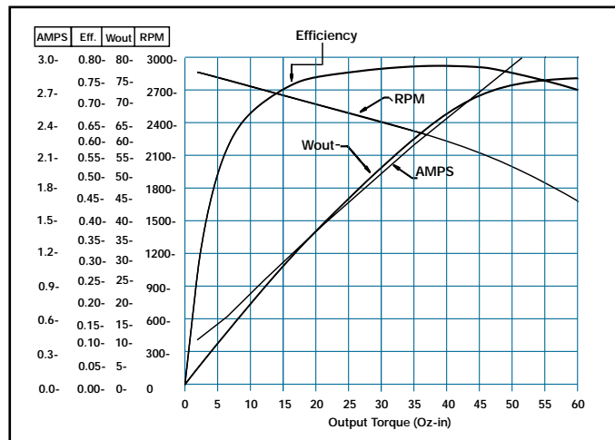
Motor Performance at 100% PWM
