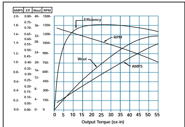
Motor Performance at 50% PWM
