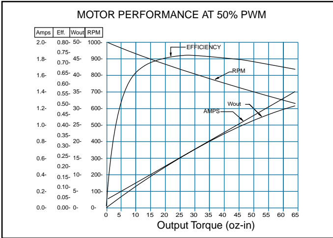
Motor Performance at 50% PWM
