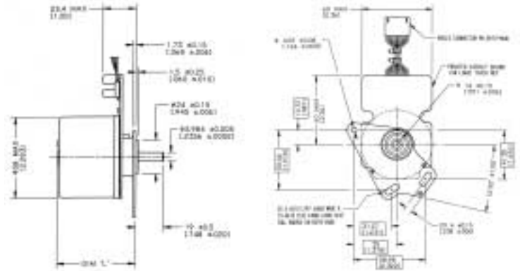
For motor length dimensions, see chart below
