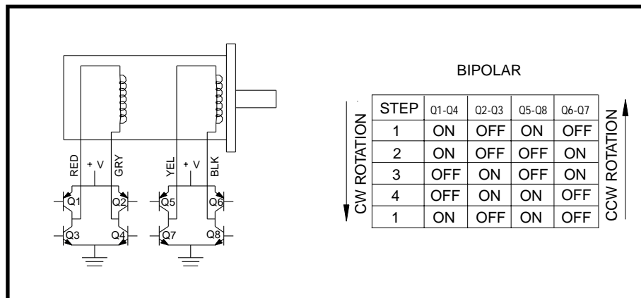
Schematic Bipolar Switching Sequence. Direction of Rotation Viewed from Shaft End.
