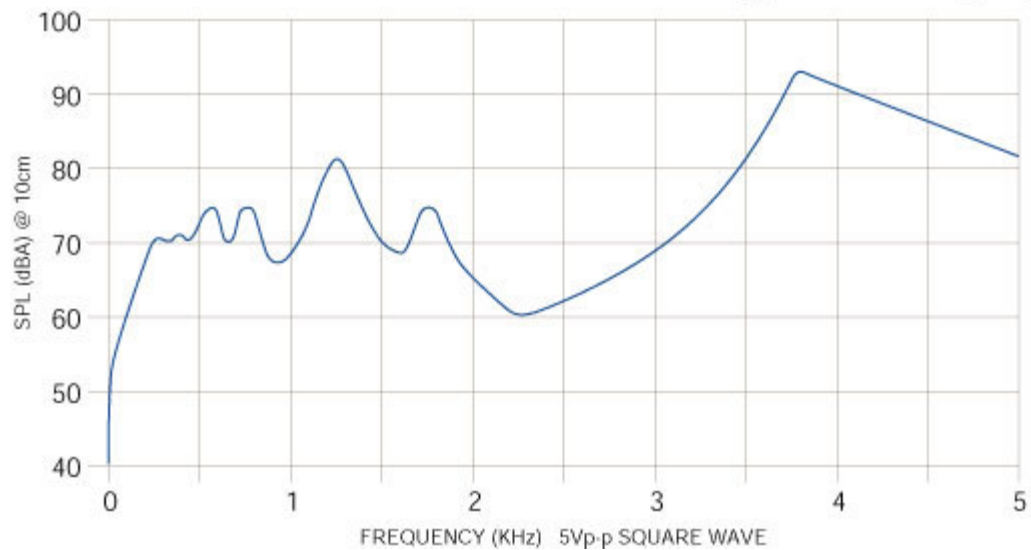
Typical SPL vs. Frequency
