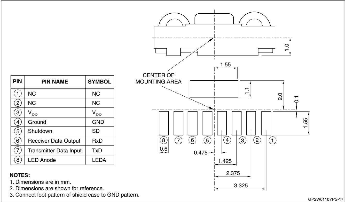
Figure 13. Recommended Footprint
