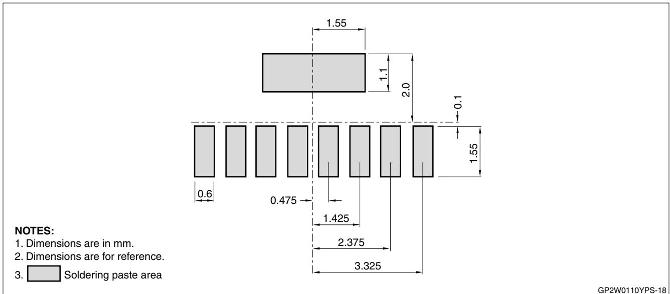
Figure 14. Recommended Solder Paste Screen Dimensions
